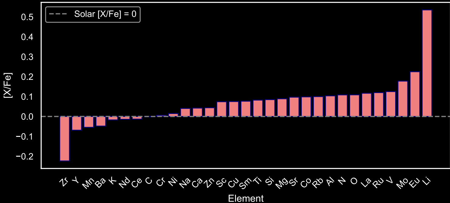
Abundance Pattern for GALAH Star Field [48] (N=293)
