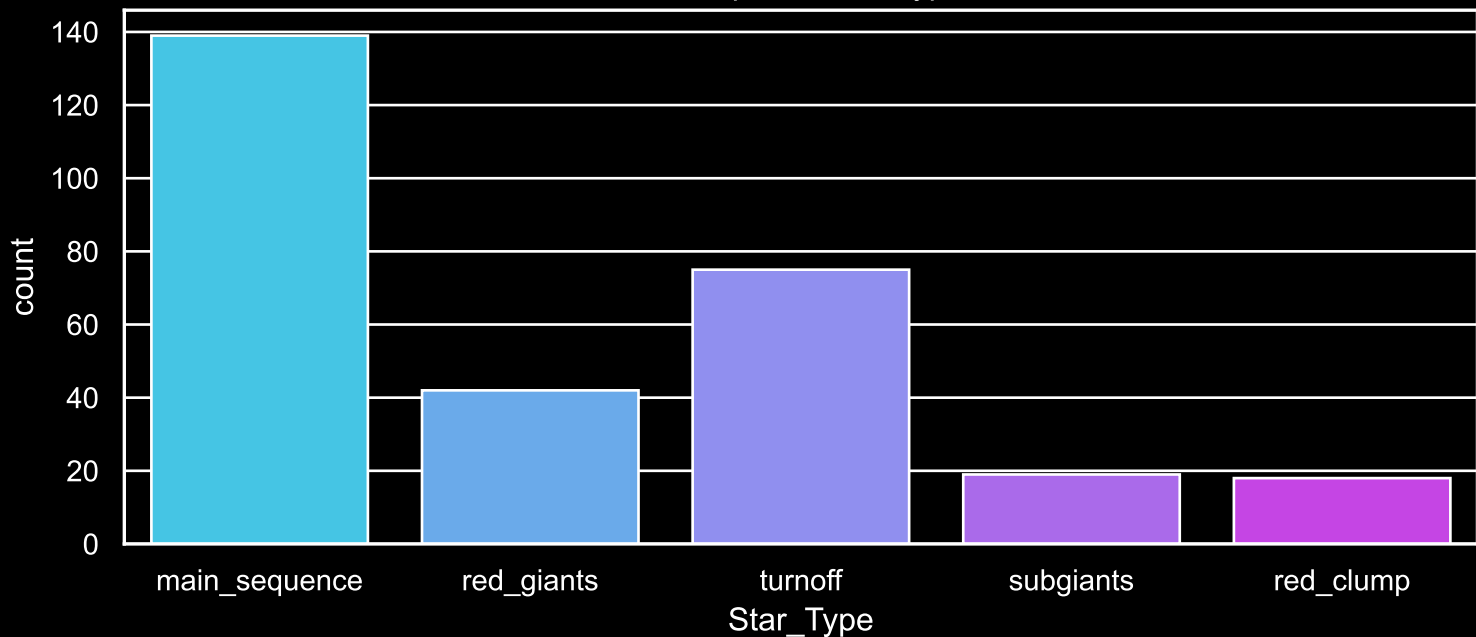
Field [48] Count plot of Star Type
