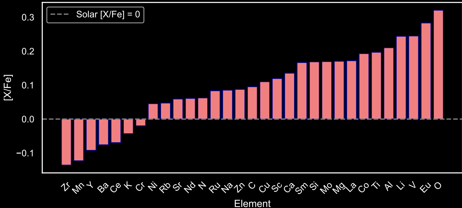
Abundance Pattern for GALAH Red Giants: Star Field [48] (N=60)
