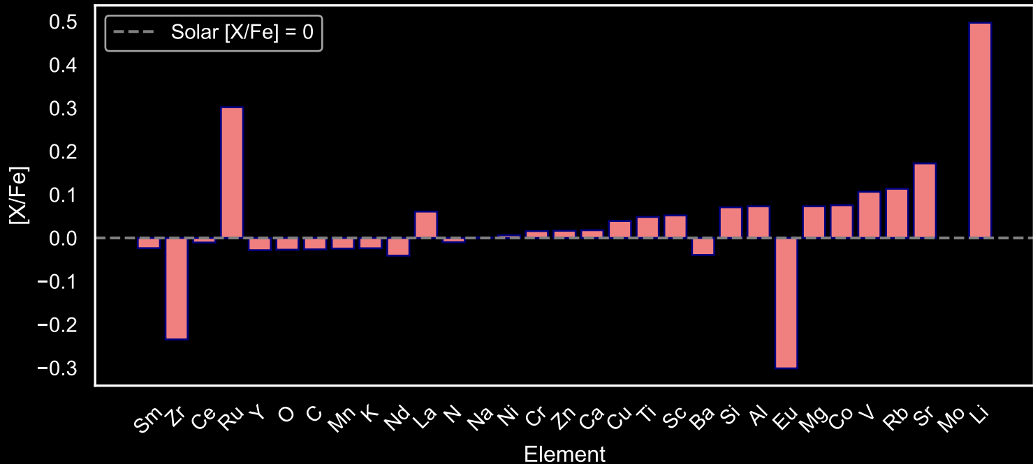
Abundance Pattern for GALAH Main Sequence Stars: Star Field [48] (N=139)
