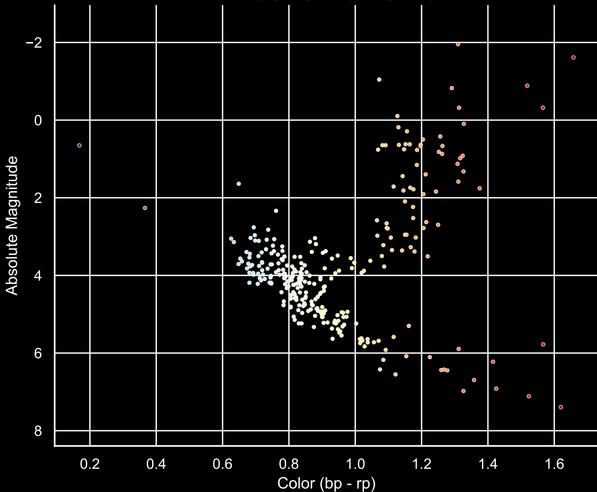
GALAH Hertzsprung-Russell Diagram Field [48] Ra [319.89] Dec [-40.06]
